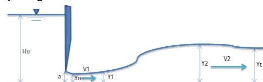
Fig. 2 Side view of the gate and the free flow condition
