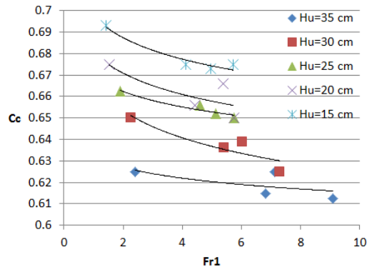
Fig. 6 Relationship between Fr1 and Cc for variable upstream level
