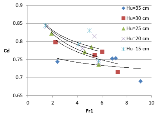
Fig. 4 Relationship between Fr1 and Cd for variable upstream level
