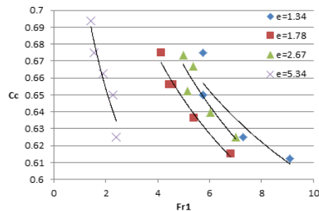
Fig. 5 Relationship between Fr1 and Cc for different values of expansion ratio
