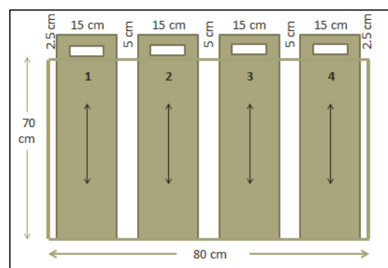
Fig. (1): An illustration of the four gates
