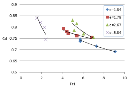
Fig. 3 Relationship between Fr1 and Cd for different values of expansion ratio
